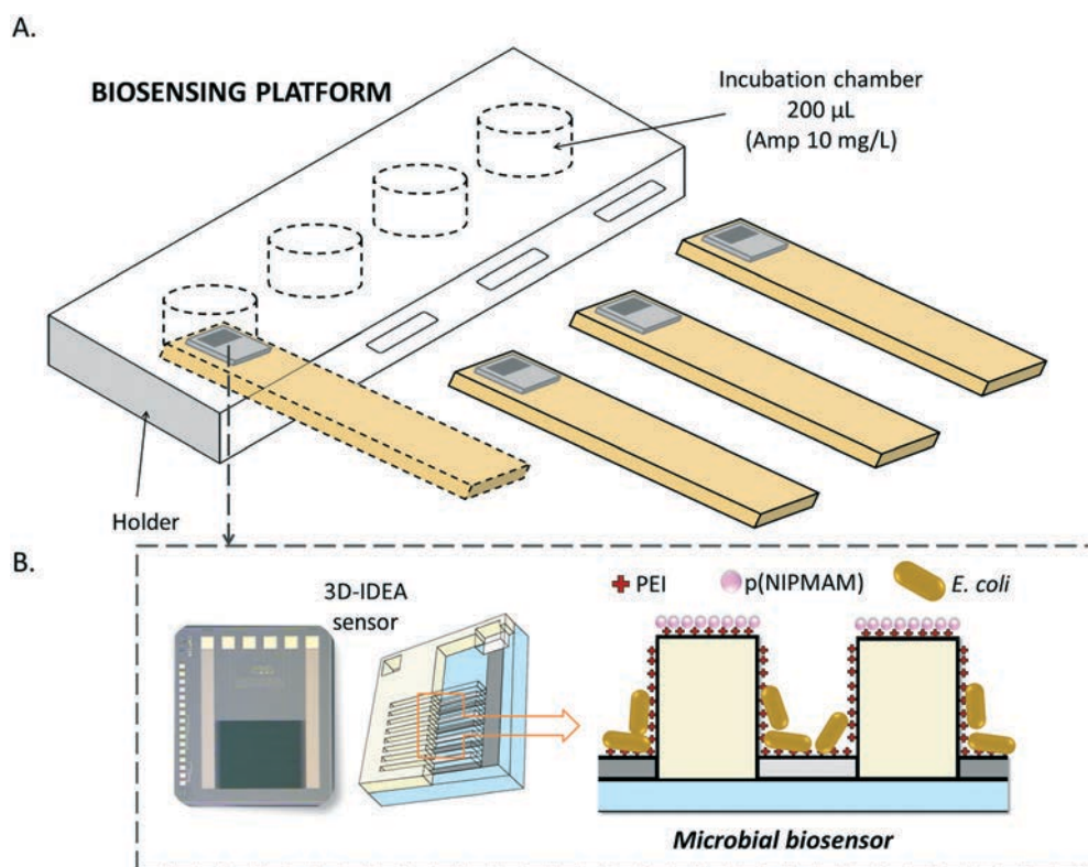
Fig. 1 (A) Biosensing platform with the integrated (B) microbial biosensors to monitor the bacterial response to ampicillin.
