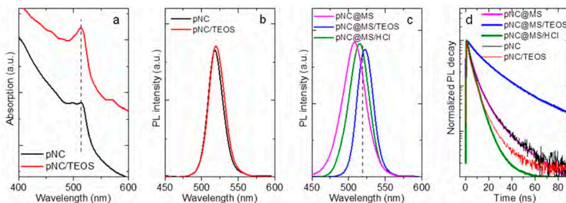
Figure 5. (a) Absorption spectra of pNC and pNC/TEOS; photoluminescence (PL) spectra of (b) pNC, pNC/TEOS and (c) pNC@MS, pNC@MS/TEOS, and pNC@MS/HCl; (d) normalized PL decay of pNC, pNC/TEOS, pNC@MS, pNC@MS/TEOS, and pNC@MS/HCl.
