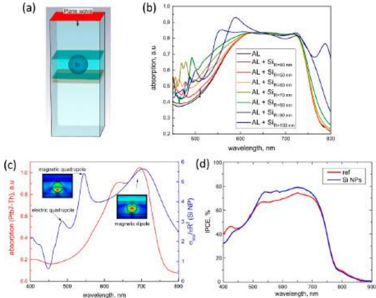
Figure 4. (a) A design for the numeral model. Red section corresponds to a port for the incident plane wave. (b) Numerically calculated spectra of absorption for the Pt7-Th absorption layer (AL) without and with Si NP of different radii, from 40 nm to 100 nm. (c) Experimentally measured absorption spectrum of Pt7-Th without Si NPs (red curve) and numerically calculated scattering efficiency of a single Si NP (with 150 nm diameter) surrounded by Pt7-Th (blue curve). Spectral peaks on the scattering spectrum correspond to different optical modes. (d) Experimentally measured incident photon-to-current efficiency (IPCE) for devices with and without Si NPs.
