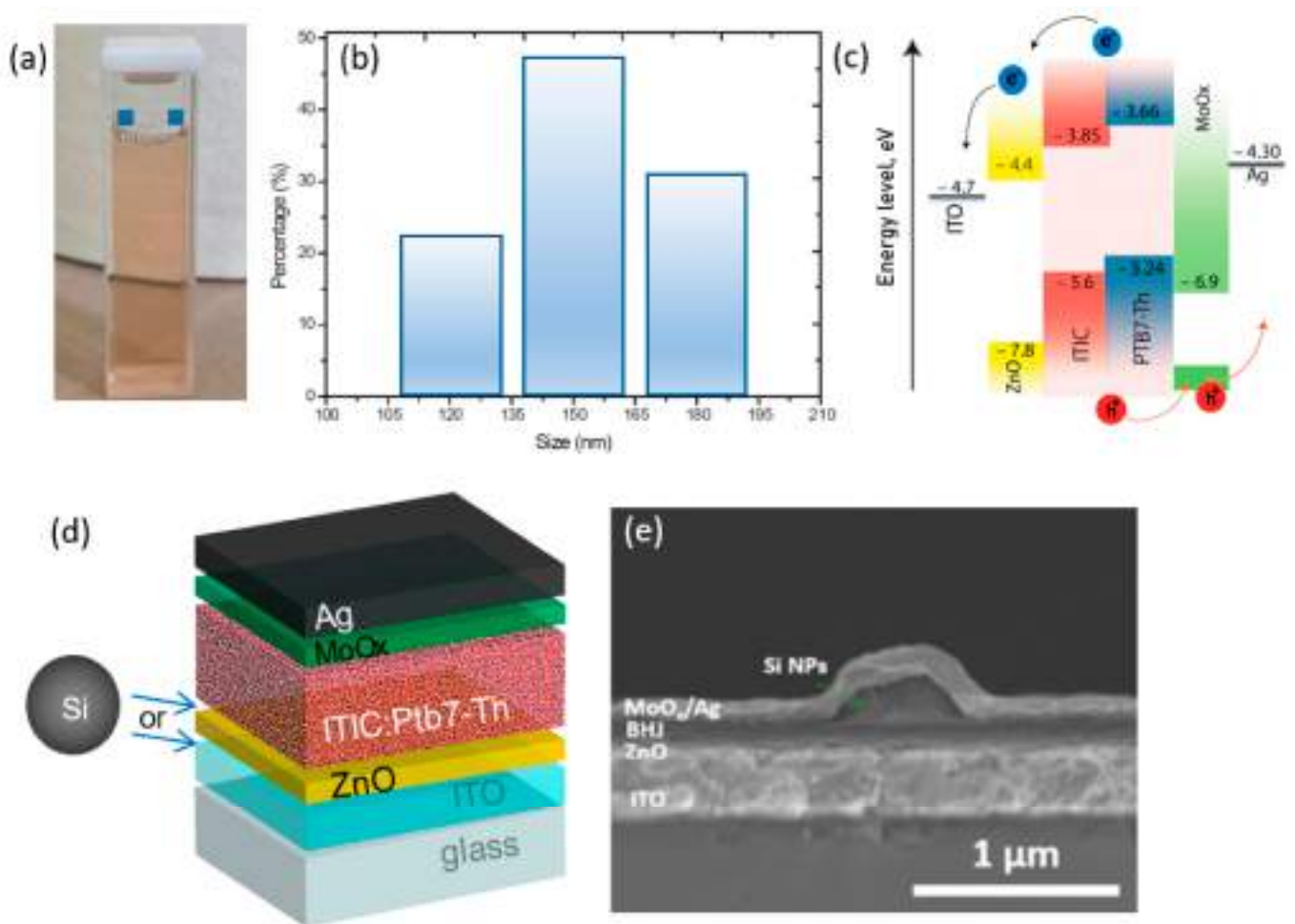
Figure 1. (a) Photo of a colloidal solution of Si NPs in isopropanol. (b) Size distribution of Si NPs in the solution. (c) Energy band diagram of the device. (d) Schematic illustration of the architecture of the studied organic solar cells. Arrows indicate the two positions of Si NPs deposition. (e) Cross-sectional SEM image of the obtained device with a single Si NP covered by BHJ/MoO x /Ag layers.
