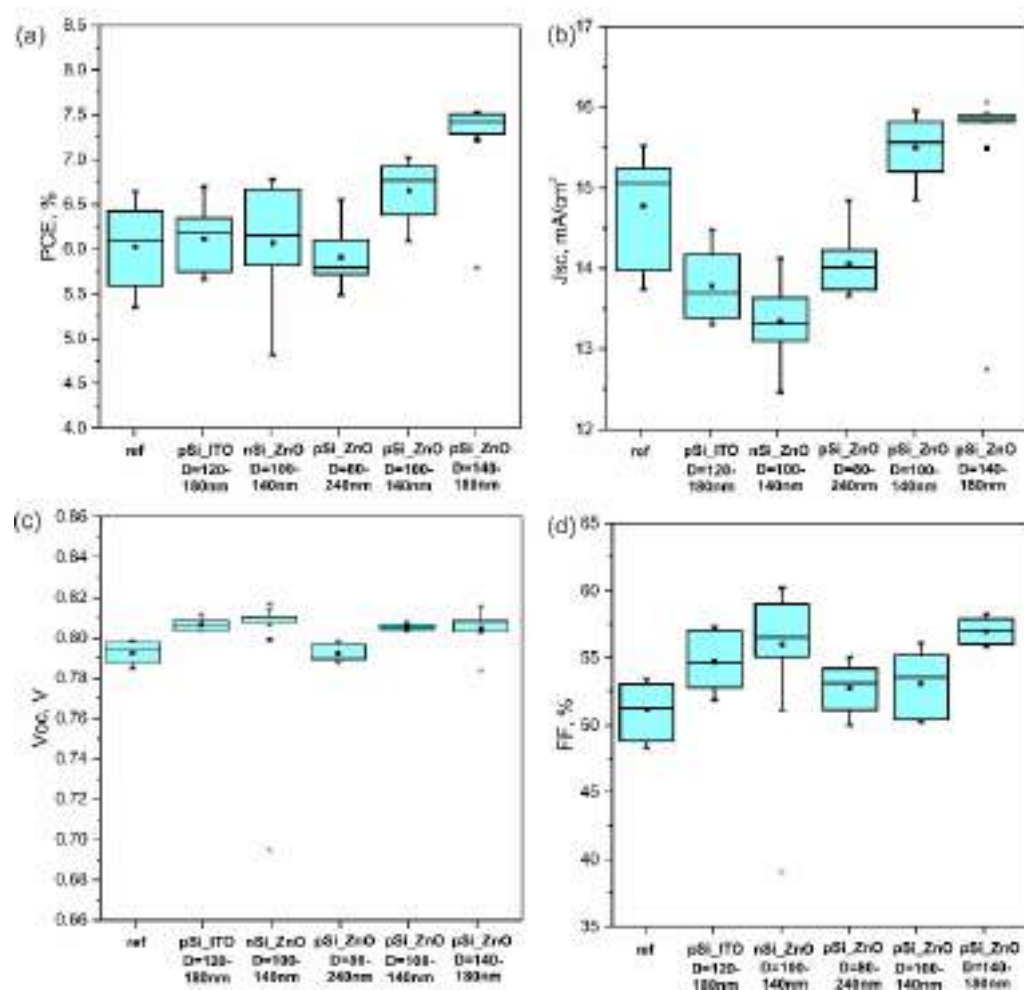
Figure 2. (a) PCE, (b) Jcs, (c) Voc, and (d) FF statistical data for photovoltaic performance of individual devices under 1 sun illumination for reference solar cells and for similar solar cells with different positions (on ITO or ZnO), diameters (D), and type of doping (nSi or pSi) of Si NPs. From left to right: reference cells without Si NPs; pSi NPs on ITO; nSi on ZnO; pSi NPs with D = 80–240 nm on ZnO deposited via spray-coating; pSi NPs with D = 100–140 nm on ZnO deposited via spin-coating with a concentration of 6 \times 10^{-4} mol L ^{-1} ; and pSi NPs with D = 140–180 nm on ZnO deposited via spin-coating with a concentration of 3 \times 10^{-4} mol L ^{-1} .
