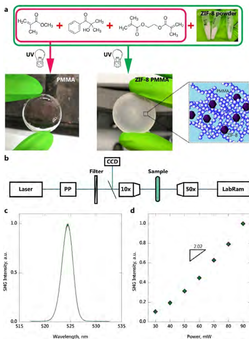
Figure 1. (a) Schematic illustration of ZIF-8– polymethyl methacrylate (PMMA) composite synthesis. (b) Optical scheme of imaging of the composite and analysis of SHG intensity. PP - pulse picker to produce 1 kHz pulse repetition rate; filter is used to tune the integral power. (c) Initial second-harmonic generation (SHG) signal of ZIF-8 powder excited by IR laser radiation (1047 nm central wavelength, 150 fs pulse duration, 50 mW, 80 MHz repetition rate) and corresponding SHG power dependence with a quadratic 2.02 \pm 0.05 slope (d).
