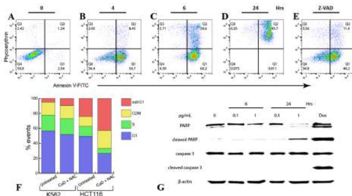
Figure 3. Death-associated events in cells treated with CuO NPs + NAC. The K562 (A–G) or HCT116 (F) cells were treated with 1 \mu g/mL CuO and 1 mM NAC for up to 24 h in the absence (A–D,F) or presence (E) of the pan-caspase inhibitor z-VAD (50 \mu M, 4h), then washed and stained with annexin V-FITC/PI (A–E) or lysed in the PI/cell cycle buffer (F) followed by flow cytometry. (G) Immunoblotting with K562 cells. See the Materials and Methods (Section 4) and text for details.
