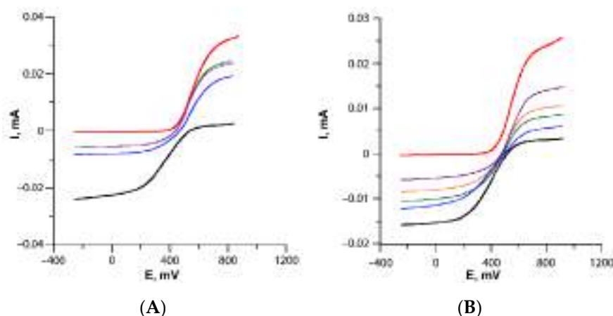
Figure 6. Voltammograms (RDE) of \text{Cu}^{+2} reduction in complex 1. (A) Mixtures of 1 and NAC in a 1:1 ratio registered successively within 25 min after mixing the reagents (blue, violet, and green curves); registered 5 min after mixing of 1 and NAC in a 1:3 ratio (red). (B) Mixtures of 1 and ascorbate in a 1:1 ratio registered successively within 100 min after mixing the reagents (blue, orange, green, and violet); registered 40 min after mixing 1 and ascorbate in a 1:3 ratio (red). Black, compound 1 alone.
