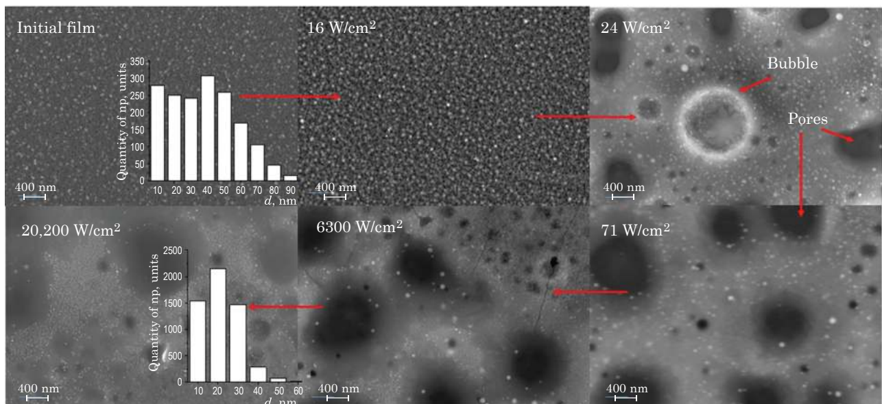
Fig. 5. SEM images of ZnO:Ag film after processing at various power densities.
