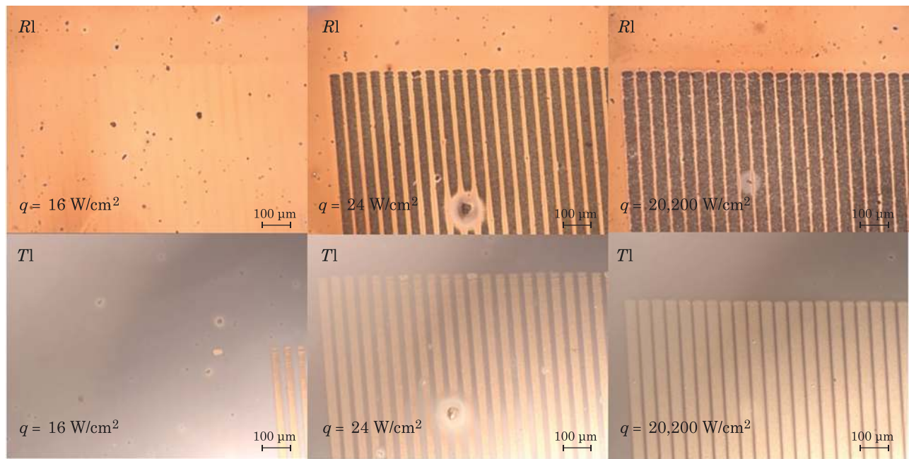
Fig. 4. Micrographs of ZnO:Ag film sections processed at different emission power densities in reflected (Rl) and transmitted light (Tl).
