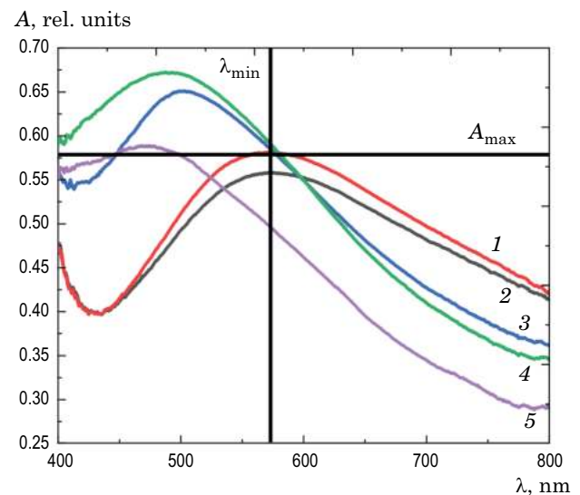
Fig. 7. Absorption spectra of the ZnO:Ag film at various power densities. Curve 1—untreated film, curve 2—16 W/cm 2 , curve 3—24 W/cm 2 , curve 4—71 W/cm 2 , and curve 5—20,200 W/cm 2 .
