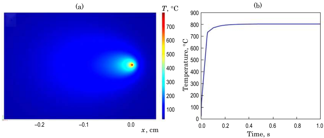
Fig. 2. Results of temperature modeling. (a) Temperature distribution over the sample's surface after 0.5 s from the start of processing at q = 71 \text{ W/cm}^2 , (b) time dependence of the temperature at the center of the laser spot on the sample surface.
