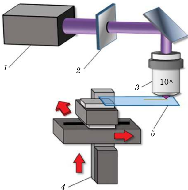
Fig. 1. Experimental scheme of laser film processing.
