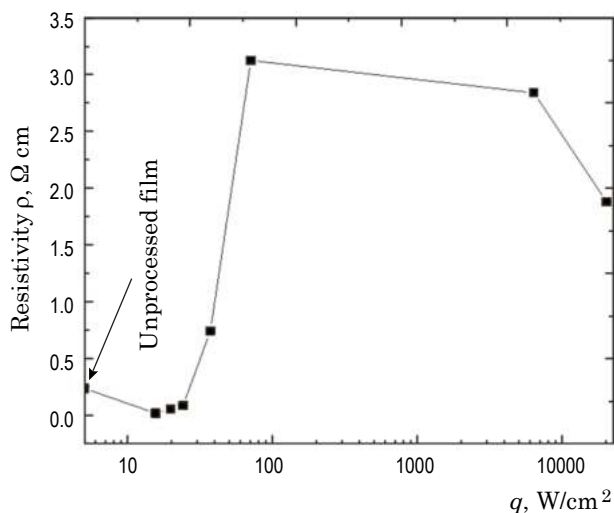
Fig. 9. Dependence of resistivity on emission power density for ZnO:Ag film annealed at 600°C. The points are connected by lines for clarity.
