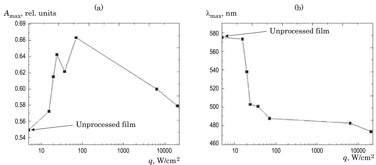
Fig. 8. Dependence of the plasmon resonance peak parameters on the power density q . (a) Dependence of A_{\text{max}} on q , (b) dependence of \lambda_{\text{max}} on q . The points are connected by lines for clarity.
