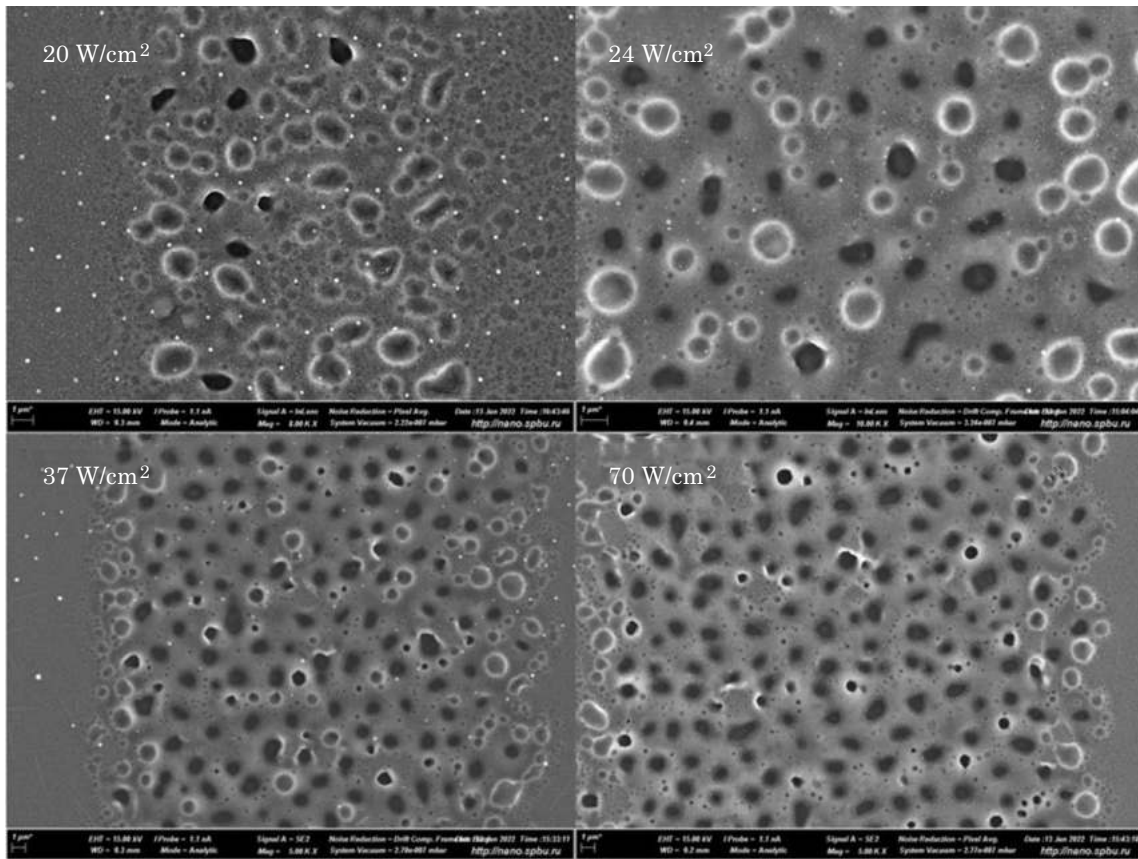
Fig. 6. Comparison of the pores and bubbles ratio on the SEM images of the ZnO:Ag film at different power densities.
