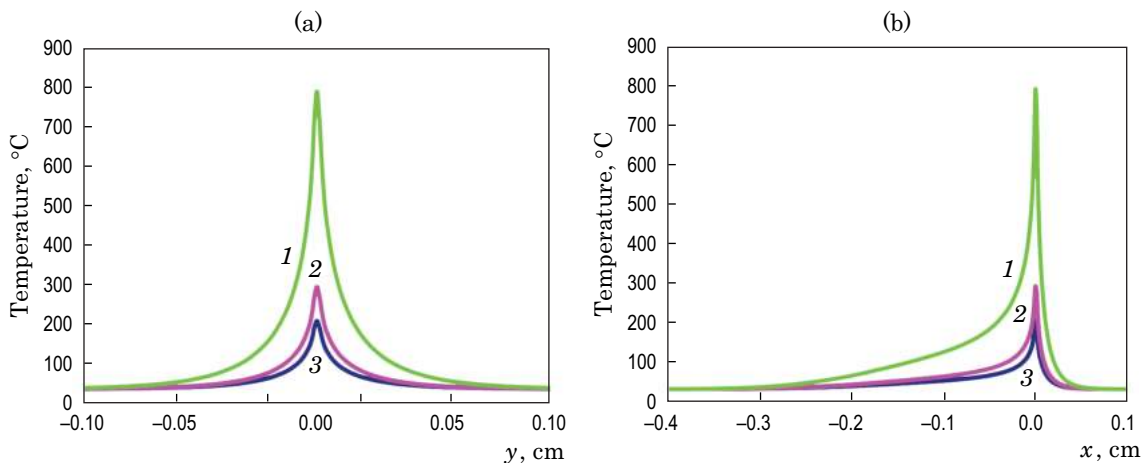
Fig. 3. Calculated temperature distribution over the surface of the sample as a result of exposure to laser radiation with a power density of 16 (curve 1), 24 (curve 2), and 71 \text{ W/cm}^2 (curve 3) 0.5 s after the start of processing. (a) Along the y -axis across the motion of the laser spot, (b) along the x -axis along the movement of the laser spot.
